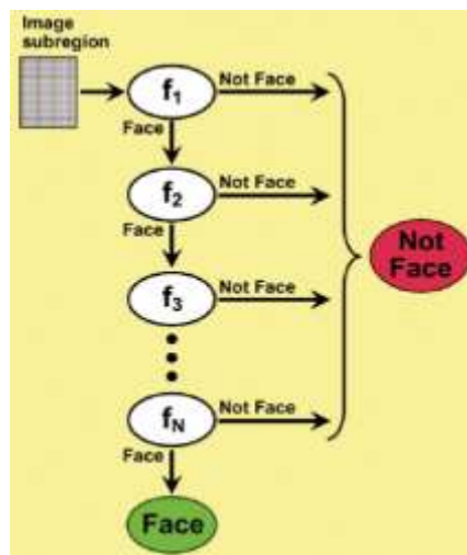
Fig :3 Face detection
